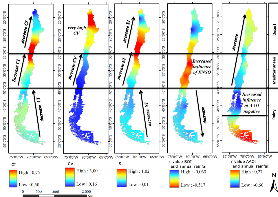
Fig. 4. Regionalization climate of Chile from CI, CV, S1, SOI and AAO.
