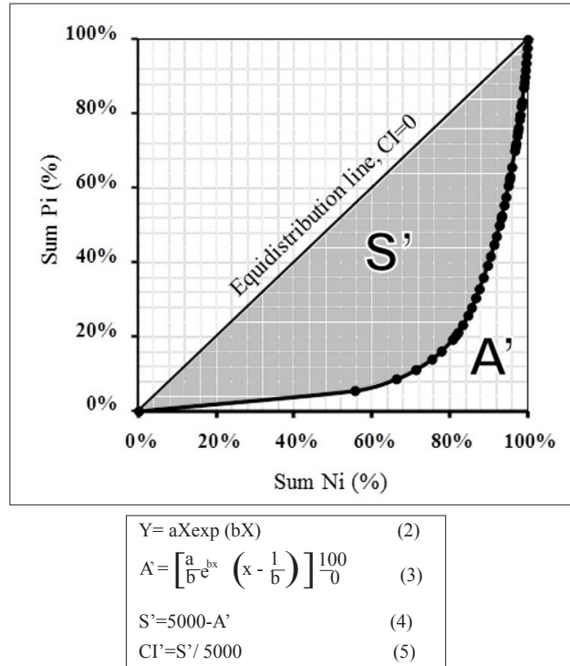
Fig. 1. Exponential curve of accumulated number of precipitation days (Sum Ni) versus amount of accumulated precipitation (Sum Pi). The solid black line represents the equidistribution line (i.e. the case in which the total precipitation is accumulated in days with equal daily precipitation accumulations).
