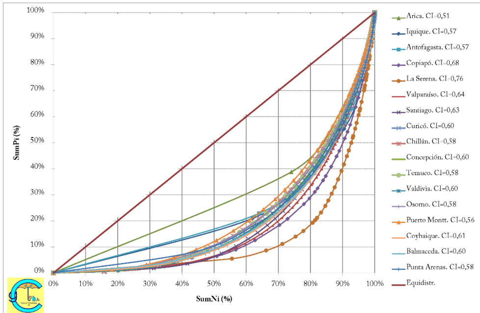
Fig. 2. Concentration curves of the 17 Meteorological stations analyzed for Chile, Period 1965-2005.
